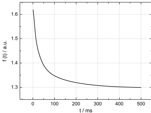
Fig. 1 The calculated conversion function f(t) between the measured mean temperature increase T_{OA} and the maximum temperature increase T_{Peak} at the center of the spot on the surface of the RPE for a rabbit fundus and a spot diameter of 130\ \mu\text{m} .
