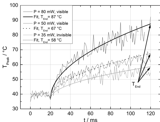
Fig. 3 Optoacoustically determined retinal temperatures T_{\text{Peak}} during laser irradiation in rabbit eyes in vivo with an irradiation time of 100 ms and a spot diameter of 130\text{ }\mu\text{m} .
