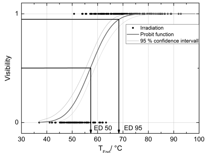
Fig. 4 Probit analysis for about 200 irradiations with different laser powers at a constant irradiation time of 200 ms in rabbit eyes in vivo (laser spot diameter 130\text{ }\mu\text{m} , P = 10\text{--}300\text{ mW} ). Visibility was evaluated one hour post treatment.
