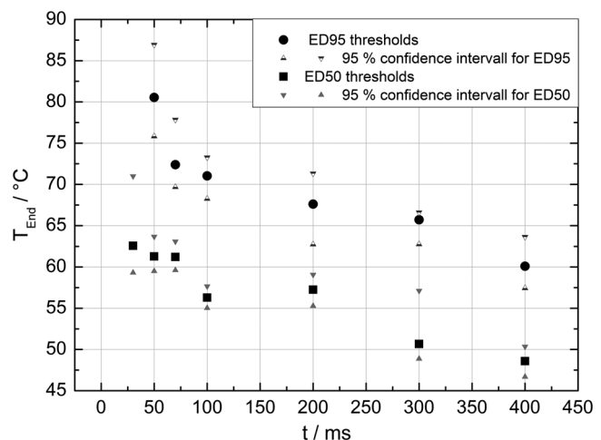
Fig. 5 Evaluated ED50 and ED95 temperature threshold values for the formation of ophthalmoscopically visible lesions (laser spot diameter 130\text{ }\mu\text{m} , P = 10\text{--}300\text{ mW} ).
