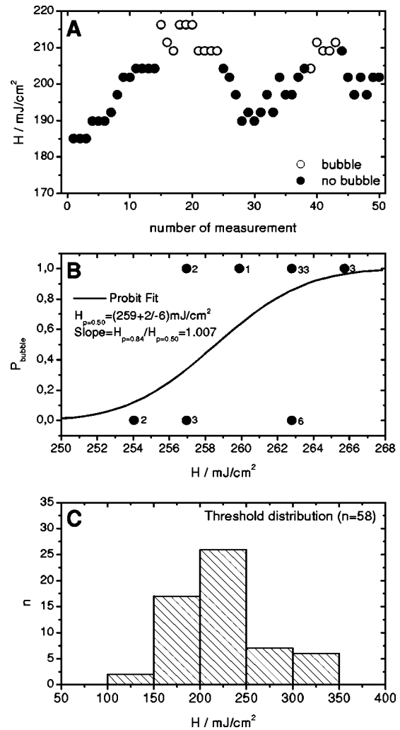
Fig. 5 Melanosomes irradiated by 240-ns pulses: (a) no hysteresis of the bubble threshold can be observed during consecutive irradiation of the same melanosome, (b) probit fit for the bubble formation threshold of an individual melanosome, which is not the same melanosome as in (a). The numbers at the data points indicate the number of measurements, which are represented by the specific point. (c) Threshold distribution for bubble formation obtained from n = 58 different melanosomes. This plot also shows, that the threshold radiant exposures for bubble formation measured for the two individual melanosomes in (a) ( H_s = 205 \text{ mJ/cm}^2 ) and (b) ( H_s = 259 \text{ mJ/cm}^2 ) are typical values.
