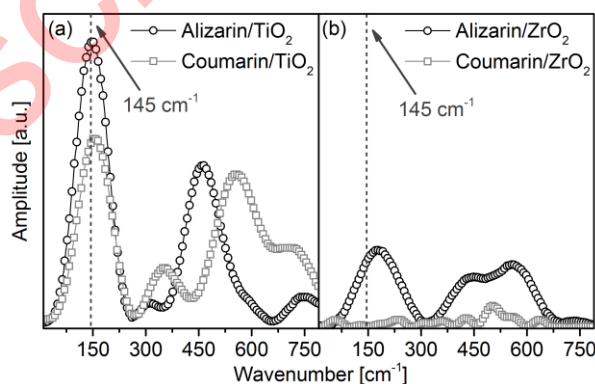
Figure 4. Fourier transformed data of (a) alizarin/ \text{TiO}_2 and coumarin/ \text{TiO}_2 samples as well as (b) alizarin/ \text{ZrO}_2 and coumarin/ \text{ZrO}_2 samples at a probe wavelength of 526 nm. The black line indicates the mode at 145\text{ cm}^{-1} .
