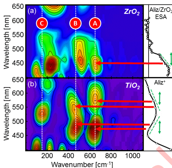
Figure 3. Fourier transformed spectra of (a) the alizarin/ ZrO_2 system and (b) the alizarin/ TiO_2 system. The three marked frequencies (“A”, “B”, “C”) assign molecular eigenmodes with their amplitude maxima (vertical lines). (a), right: Excited state absorption band obtained from transient absorption measurements on alizarin/ ZrO_2 (see ref. 12); (b), right: absorption spectrum of alizarin cation (see ref. 8). The arrows indicate which peak in the 2D plots correspond to the respective slopes in the absorption spectra.
