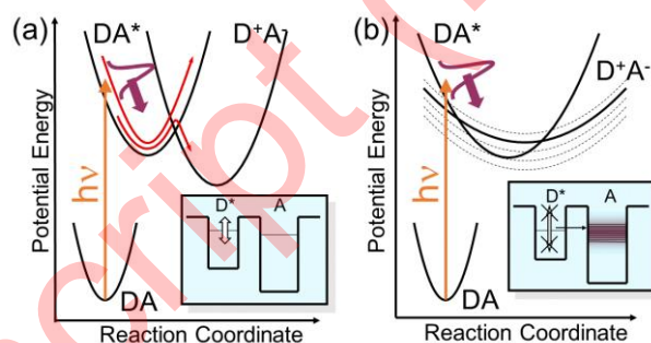
Figure 1. Sketch of (a) bimolecular ET and (b) ET at molecule/semiconductor interfaces in the potential energy surface and the electronic quantum dot picture (inset).
