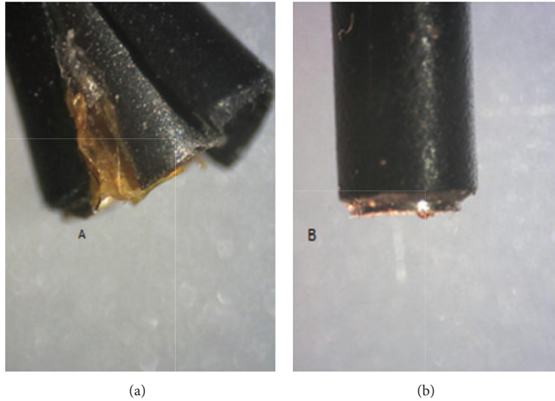
FIGURE 4: Destroyed (a) and intact (b) probes of the electrohydraulic device (magnification of 60).
